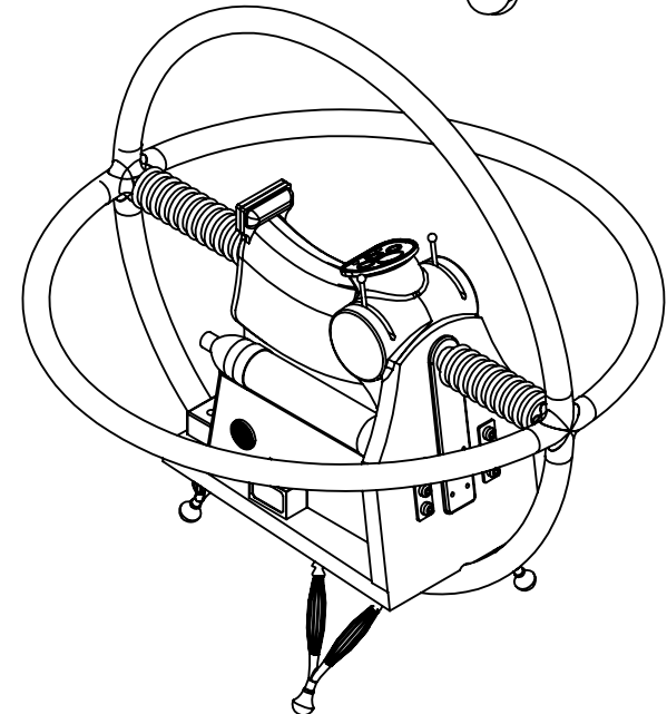
Ring Assembly
