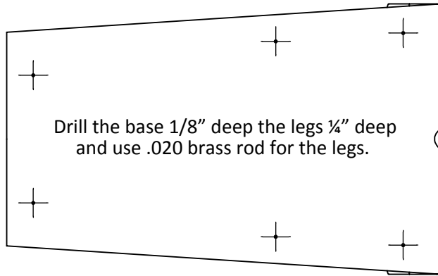
Leg Placement Drill Guide
